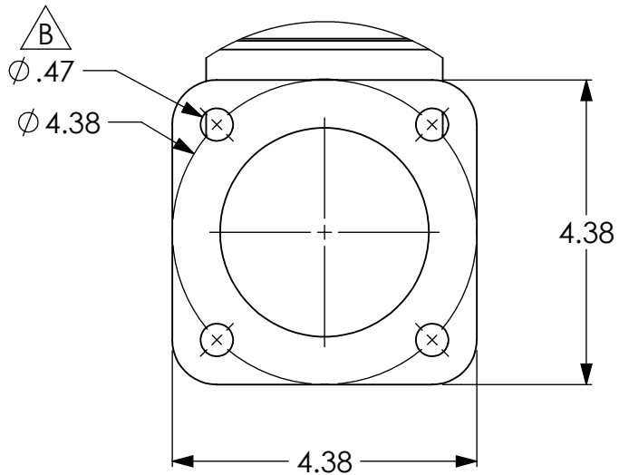
FLANGE DETAIL A (Typ 3 Places)
